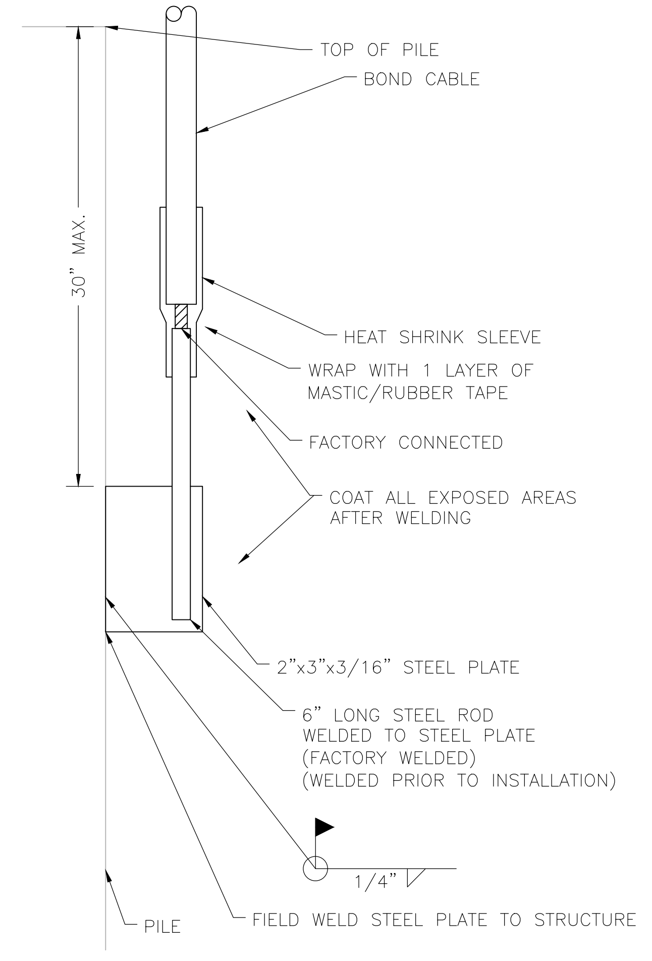
BOND CABLE CONNECTION SCALE: NONE
